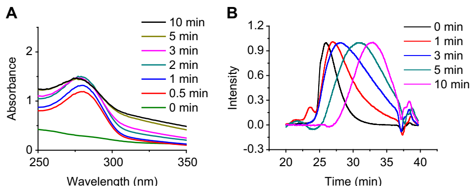
Fig. 2. Light-triggered degradation of PBAEs. UV–Vis spectra (A) and GPC curves (B) of P1-13700 after UV irradiation ( \lambda = 365 nm, 20 mW/cm 2 ) for various time.
