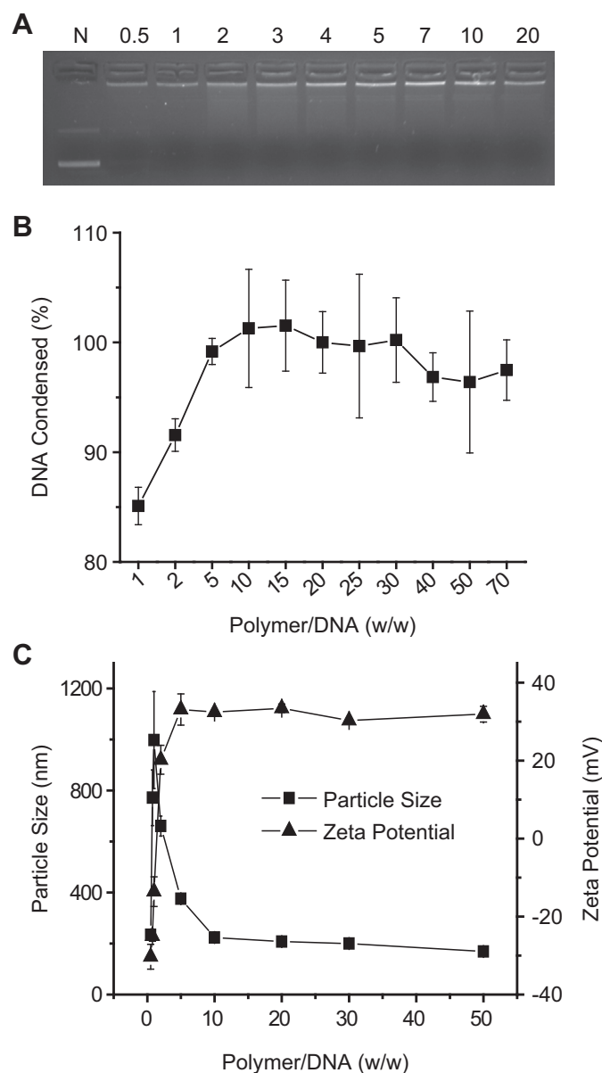
Fig. 3. Characterization of PBAE/DNA polyplexes. DNA condensation by P1-13700 at different polymer/DNA weight ratios as evaluated by the gel retardation assay (A) and the EB exclusion assay (B). N represents naked DNA in (A). (C) Size and zeta potential of P1-13700/DNA polyplexes.
