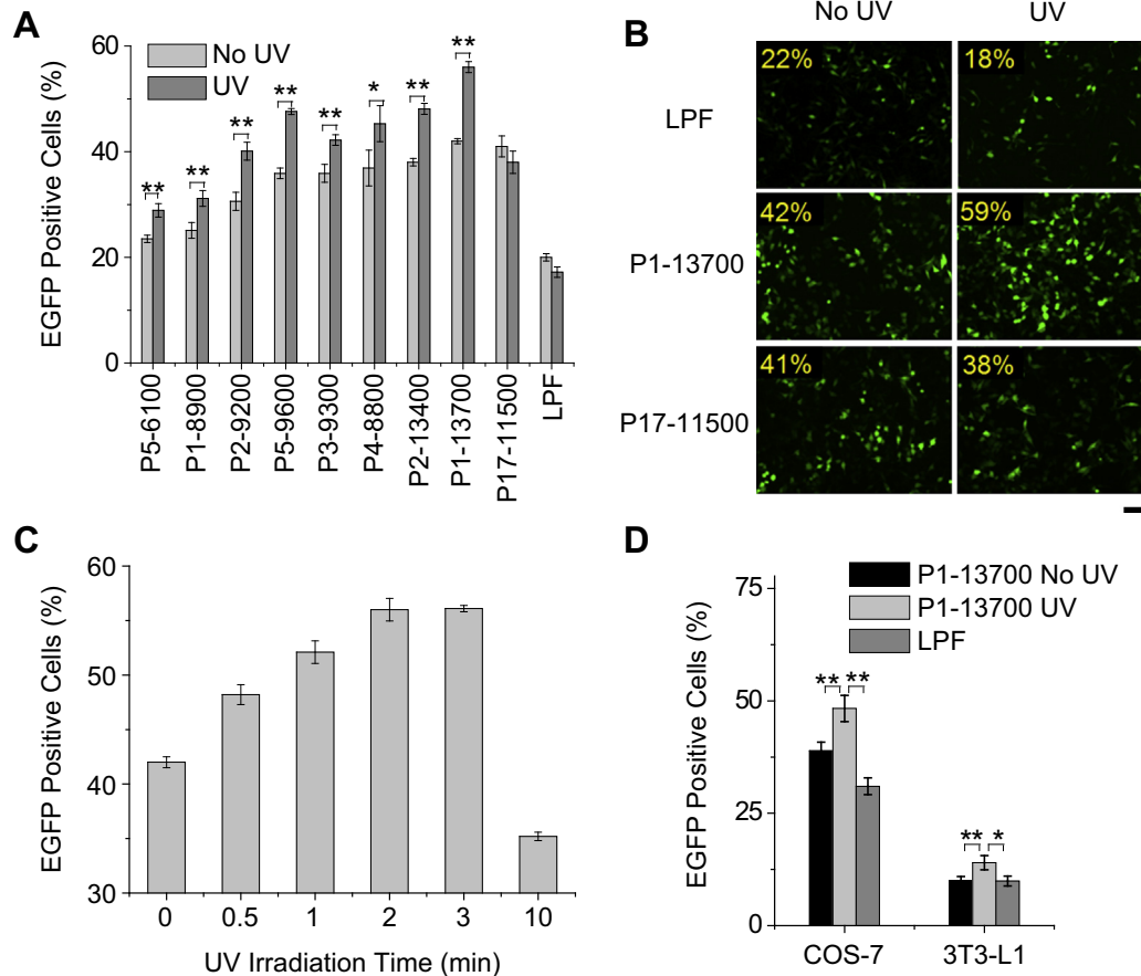
Fig. 5. Light-responsive transfection capabilities of PBAE/DNA polyplexes (weight ratio of 50). (A) A comparison of transfection efficiencies of PBAE/DNA polyplexes in HeLa cells in response to UV irradiation ( \lambda = 365 nm, 20 mW/cm 2 ) for 2 min. Results were represented as percentage (%) of EGFP-positive cells ( n = 3 ). (B) Fluorescence images of transfected HeLa cells w/ and w/o UV irradiation. Bar represented 50 \mu m. (C) Effect of UV irradiation time on the transfection efficiencies of P1-13700/DNA polyplexes ( n = 3 ). Laser power was fixed at 20 mW/cm 2 ( \lambda = 365 nm). (D) Enhanced transfection efficiencies of P1-13700/DNA polyplexes in COS-7 and 3T3-L1 cells in response to UV irradiation for 2 min ( \lambda = 365 nm, 20 mW/cm 2 , n = 3 ).
