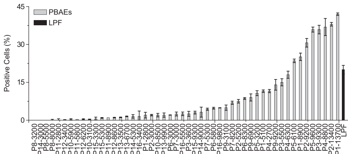
Fig. 1. Transfection efficiencies of PBAEs with various side charged groups in HeLa cells. Results were represented as percentage (%) of EGFP-positive cells.
