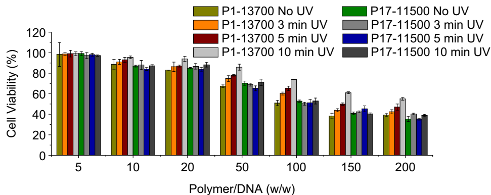
Fig. 7. Viabilities of HeLa cells transfected with polyplexes at various polymer/DNA weight ratios and irradiated with UV light ( \lambda = 365 nm, 20 mW/cm 2 ) for different time periods ( n = 3 ). Cells were treated with polyplexes for 4 h, irradiated with UV light, and further cultured for 48 h before viability assessment using the MTT assay.
