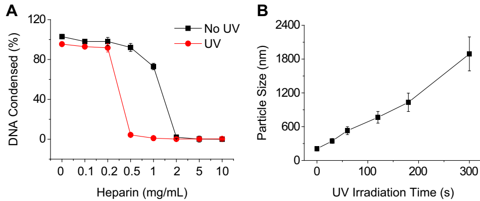
Fig. 4. Light-triggered polyplex dissociation and DNA release. (A) DNA release from UV-irradiated and non-irradiated P1-13700/DNA polyplexes in the presence of heparin at various concentrations ( n = 3 ). (B) Alteration of P1-13700/DNA polyplex diameter upon UV irradiation ( \lambda = 365 nm, 20 mW/cm 2 ) for different time periods as measured by DLS.
