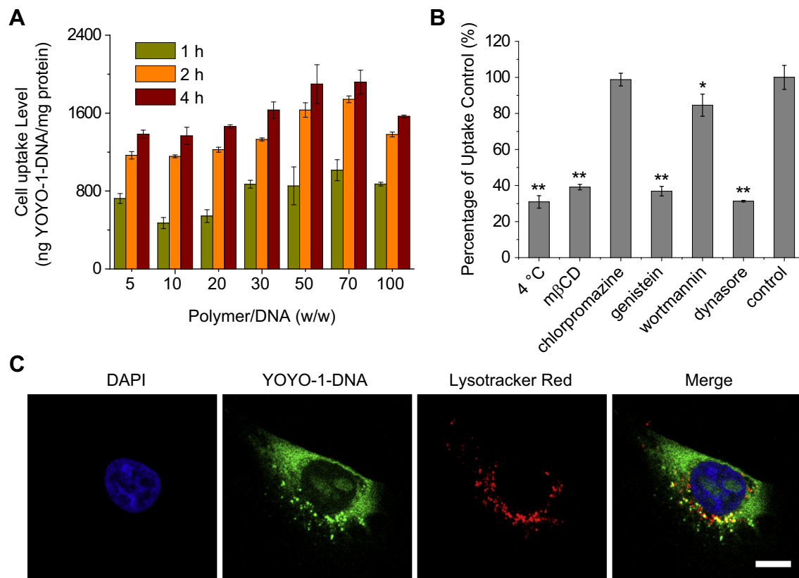
Fig. 6. Intracellular kinetics of P1-13700/YOYO-1-DNA polyplexes (weight ratio of 50) in HeLa cells. (A) Uptake level of polyplexes following incubation at 37 °C for different time ( n = 3 ). (B) Uptake level of polyplexes at 4 °C or in the presence of various endocytic inhibitors. Results were represented as percentage (%) of the uptake level at 37 °C and in the absence of inhibitors ( n = 3 ). (C) CLSM images showing the cellular internalization and distribution of polyplexes in HeLa cells following incubation at 37 °C for 4 h. Cell nuclei were stained with DAPI and the endosomes/lysosomes were stained with LysoTracker Red. Bar represented 10 \mu m.
