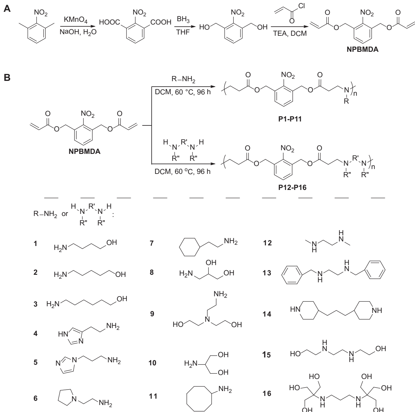
Scheme 1. Synthesis of (2-nitro-1,3-phenylene)bis(methylene) diacrylate (A) and a library of photo-responsive PBAEs (P1–P16) with various side charged groups (B).
