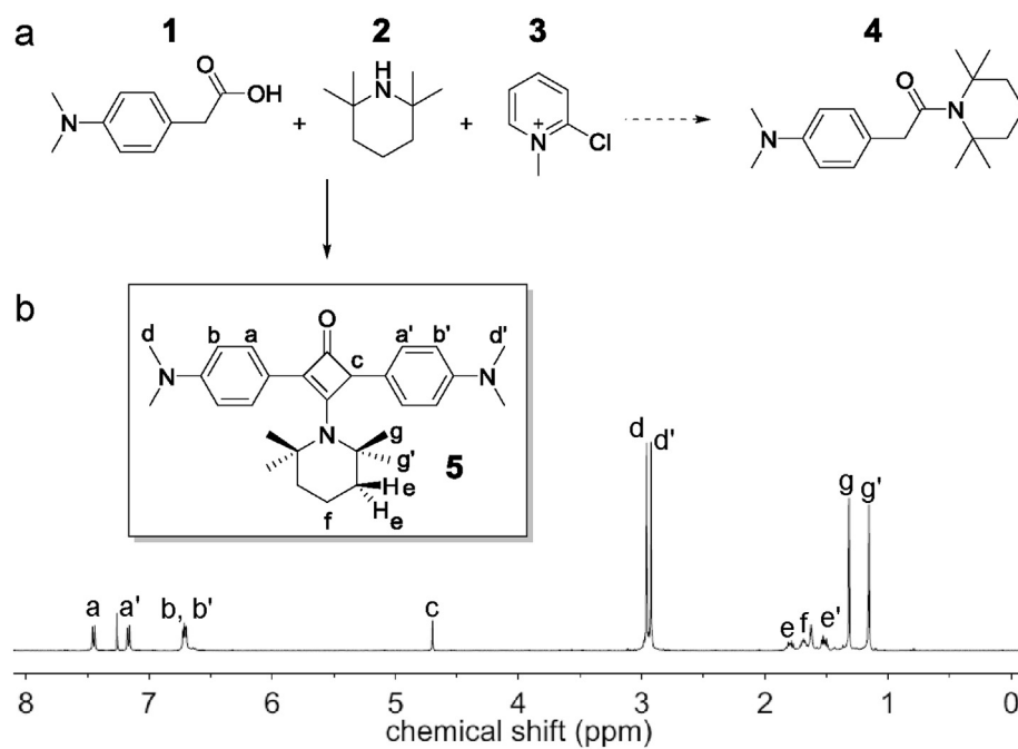
Fig. 1. Amidation reaction gives unexpected product: (a) Amidation reaction of 1 and 2 gives reductive squaraine derivative 5 instead of expected amide 4 as the major product; (b) 1 H NMR spectrum of 5 (peaks were assigned to corresponding protons).
