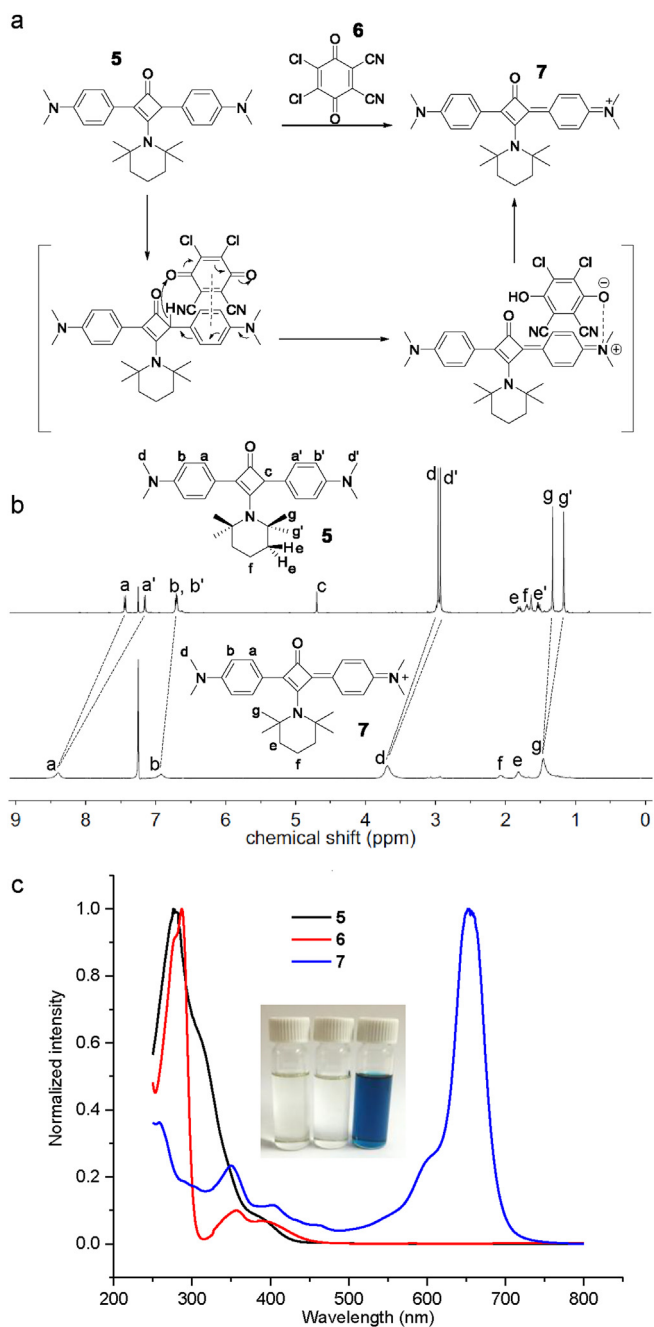
Fig. 2. Oxidation of 5 by DDQ: (a) Scheme showing oxidation of 5 by DDQ with the proposed synergistic hydride transfer mechanism; (b) Comparison of ^1\text{H} NMR spectra of 5 (asymmetric reductive form) and 7 (symmetric oxidative form); (c) UV–Vis absorption spectra of 5 , 6 , and 7 ; Inset: images of solutions of 5 , 6 , and 7 showing significant color change before and after mixing of 5 and 6 (all solutions were characterized in the concentration of 10^{-4} M).
