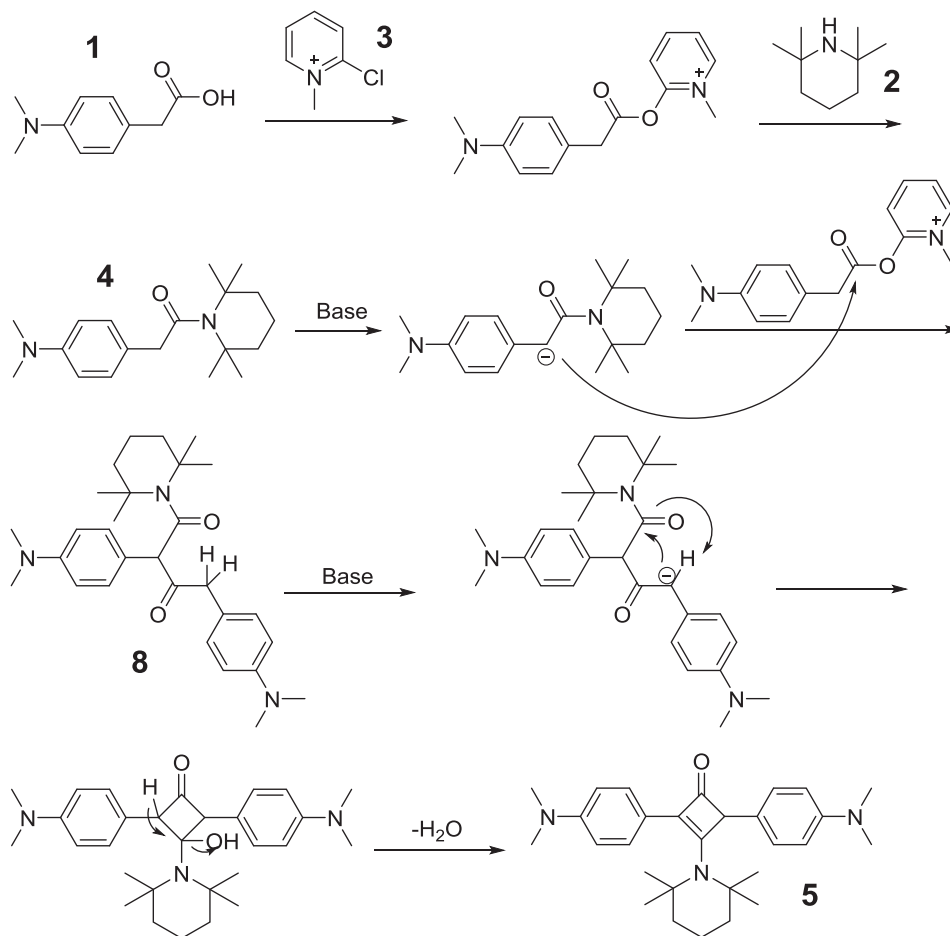
Scheme 2. Proposed mechanism for the synthesis of reduced form of aminosquaraine 5 .
