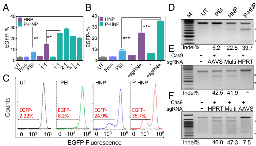
Fig. 3. In vitro gene disruption. (A) EGFP disruption assay of Cas9 expression plasmid and sgRNA expression plasmid delivery by HNPs or P-HNPs in U2OS.EGFP reporter cells. The ratios in the figure are weight ratios for Cas9 expression plasmid:sgRNA expression plasmid. (B and C) EGFP disruption assay of Cas9 expression plasmid and in vitro-synthesized sgRNA delivery in U2OS.EGFP reporter cells. Short dash under the bars in B indicates the group treated by only Cas9 expression plasmids. (D–F) GCD assay of indels in the EGFP gene in U2OS.EGFP cells (D), the AAVS1 gene in HEK293T cells (E), and the HPRT1 gene in HEK293T cells (F). “Multi” is the group treated by Cas9 expression plasmid delivery and subsequent codelivery of AAVS1- and HPRT1-targeting sgRNAs. Arrows indicate the cutting products. Free, treatment with naked nucleic acids; UT, untreated group.
