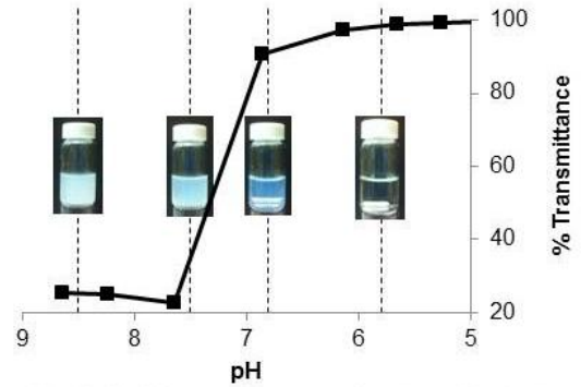
(b) Turbidity measurements when titrated
